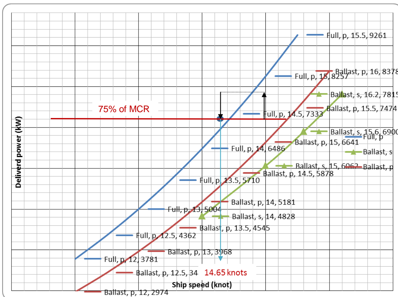
Figure 3.1: Power curves
